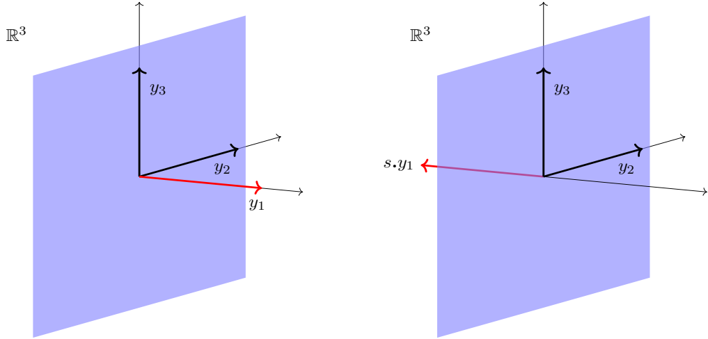
Figure 1.1.B: Diagram of a real reflection in \mathbb{R}^3 from Example 1.1.8. The shaded area represents the hyperplane \text{Fix}_{\mathfrak{h}}(s) = \ker(1-s) = \text{span}\{y_2, y_3\} = \ker(x_1) .
