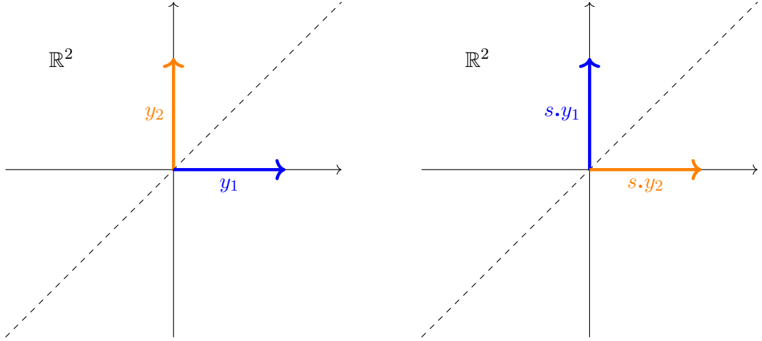
Figure 1.1.A: Diagram of a real reflection from Example 1.1.3. Points along the dashed line are fixed by s and the rest of the plane is reflected across that axis.
